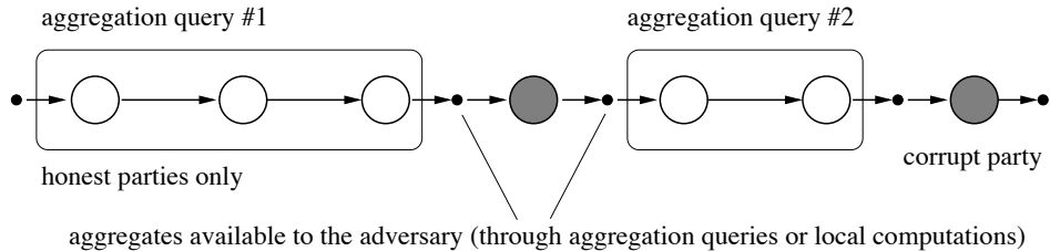
Figure 1: Example of a trivial combination of replies to aggregation queries and local computations by corrupt parties.
