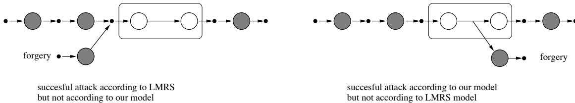
Figure 3: Comparison of the LMRS security model and our (strong) model: Prepending any values by corrupt parties is not considered a successful attack in our model (left part), whereas branching into a different sequence from some intermediate value is not considered a successful attack in the LMRS model (right part).
